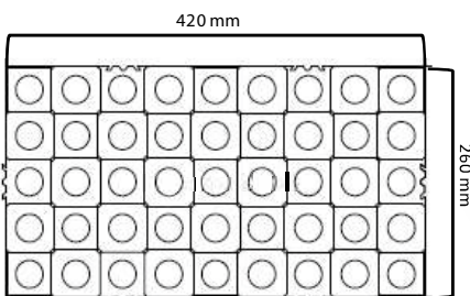
Detail: integrated connectors
